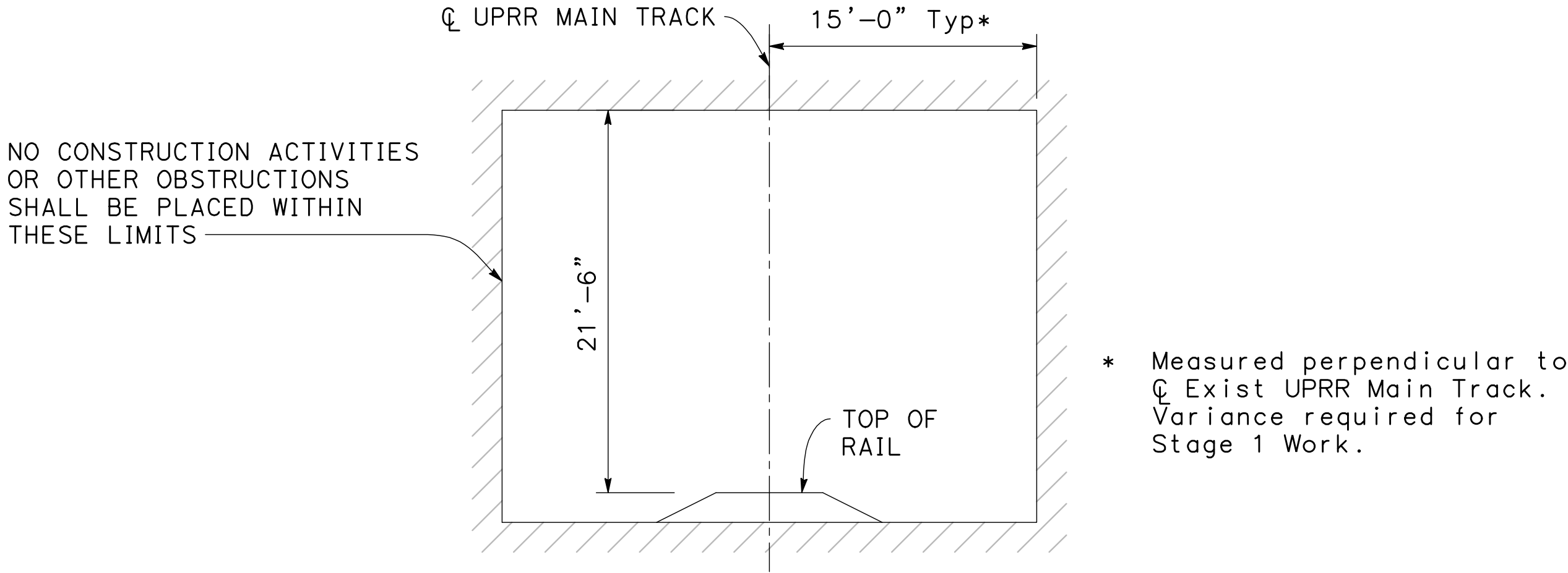
MINIMUM TEMPORARY CONSTRUCTION CLEARANCE DIAGRAM
